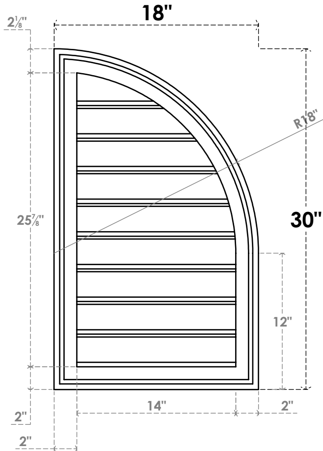
FRONT
